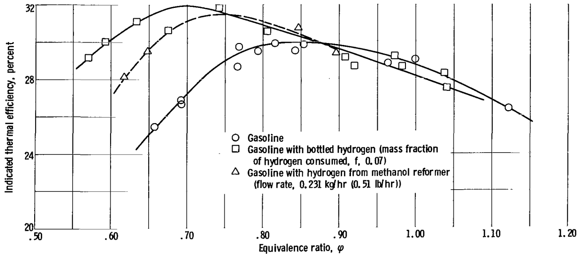
Figure 11. - Indicated thermal efficiency as function of equivalence ratio. Engine speed, 2140 rpm; brake horsepower, 27 kW (36 bhp).
